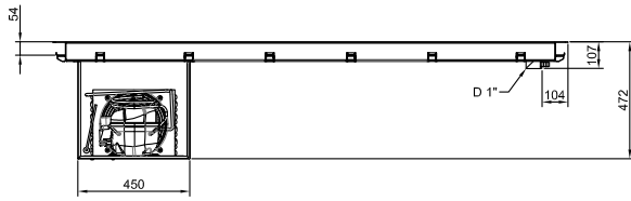
Lateral
